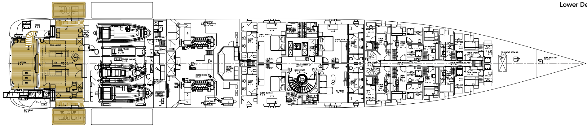
Lower Deck
