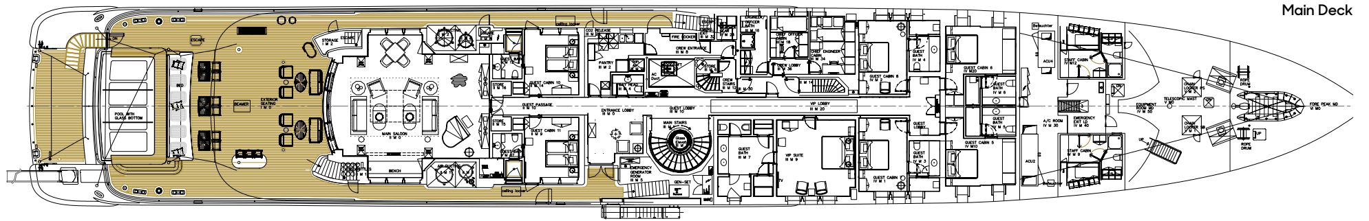
Main Deck
